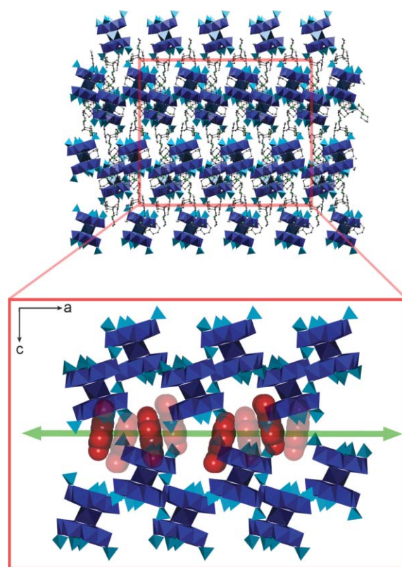
Fig. 3 Representation of the BTC-filled channels in 1 . Top: View along the crystallographic b axis. Bottom: Cross-section through the channels. Emphasised in red, space-filling representation: stacked BTC molecules. The green arrow indicates the directionality of the channels. Sparteine and water molecules are omitted for clarity.
