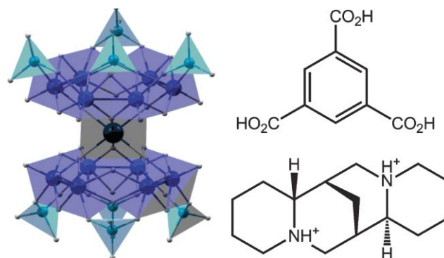
Fig. 1 Building blocks used in the synthesis of compound 1 . LHS: Polyhedral representation of the dimer {Mo 6 } 2 ( 1a ): blue octahedra: MoO 6 ; light blue tetrahedra: PO 4 ; dark blue octahedron: NaO 6 . Blue spheres: Mo, dark blue sphere: Na, light blue spheres: P, small white spheres: O. RHS: Top: 1,3,5-benzenetricarboxylic acid, (H 3 BTC). Bottom: di-protonated (–)-sparteine. This colour scheme will be used throughout the text.
