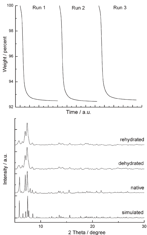
Fig. 4 Top: TGA water desorption showing three consecutive runs with a weight loss of 7.5 wt.%. Bottom: Powder X-ray diffraction patterns of 1 as simulated from single crystal XRD (123 K), native material, after dehydration and after rehydration (room temperatures).
