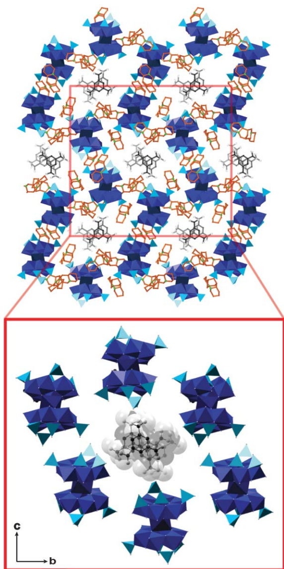
Fig. 2 Top: Representation of the crystal lattice of 1 along the crystallographic a axis. The (–)-sparteine cations are highlighted in brown and show the chiral environment into which the BTC is bound. Bottom: Illustration of the hexagonal 1D channels in 1 . The staggered arrangement of the BTC molecules is clearly visible. Sparteine and water molecules are omitted for clarity.
